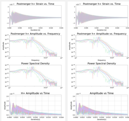
Figure 1: Analytical waveforms of 10 post-mergers selected from the posterior samples.
